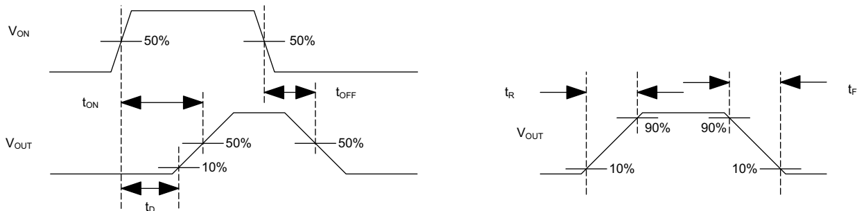
Figure 22. Timing Waveforms
